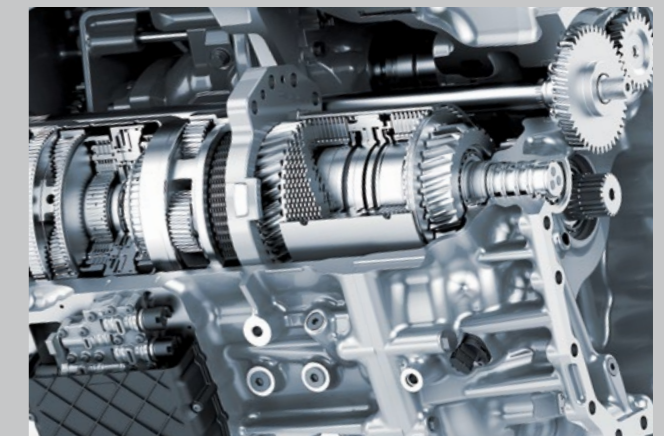
Continuously variable TTV transmission with a speed range from 0.2 to 60 km/h at reduced engine speed. Perfect precision.
